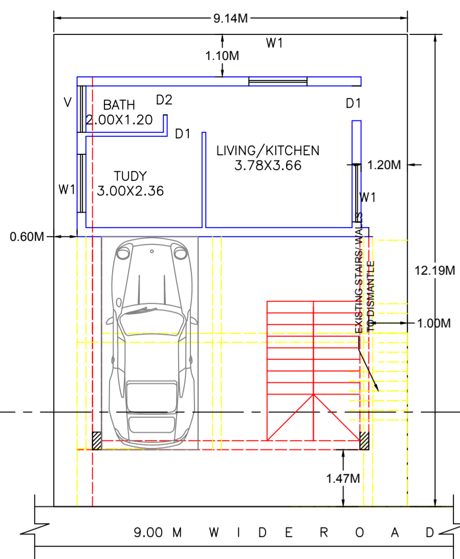
EXISTING GROUND FLOOR PLAN & PROPOSED ADDITIONS/ ALTERATIONS(1:100)
