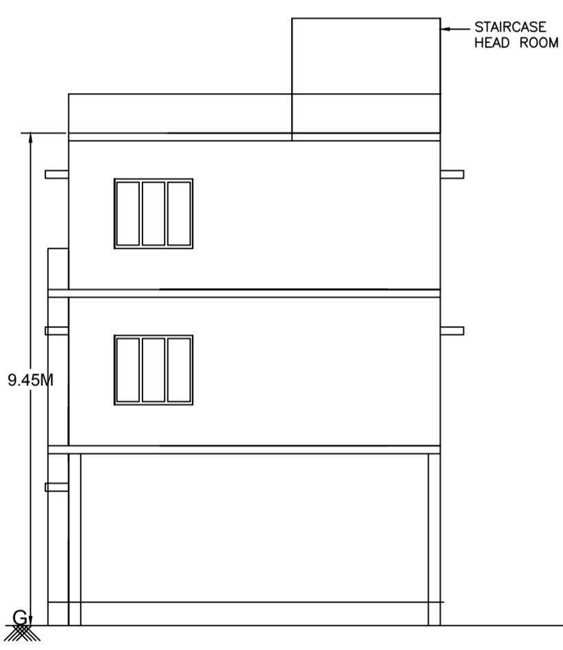
ELEVATION(1:100)
