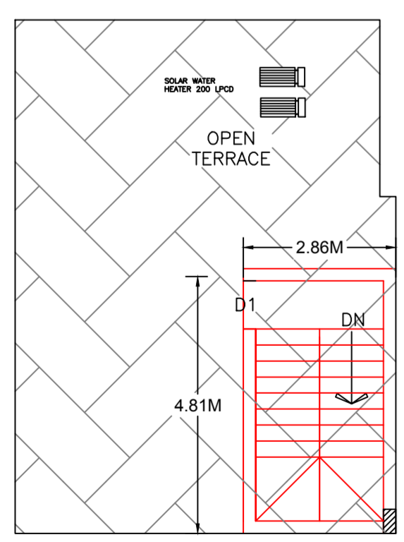
PROPOSED TERRACE FLOOR PLAN (1:100)
